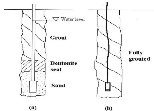
Figure 3: Traditionally piezometer and fully grouted piezometer, Mikkelsen & Green 2003
